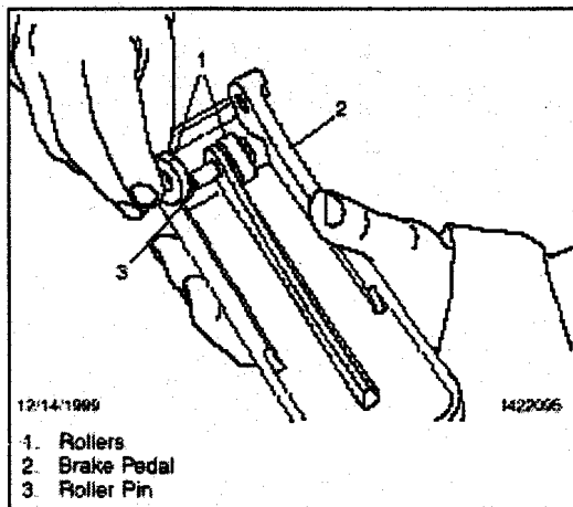
Fig. 3. Roller Pin Replacement
