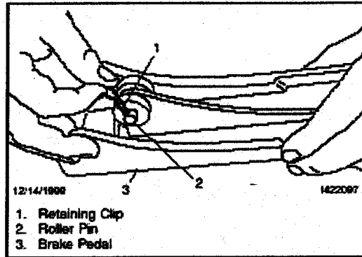
Fig. 2. Remove the Retaining Clip
