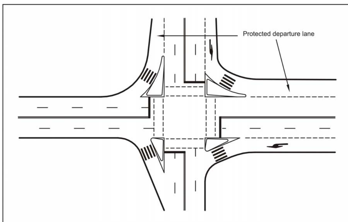
Figure 5.2 Corner island treatments
