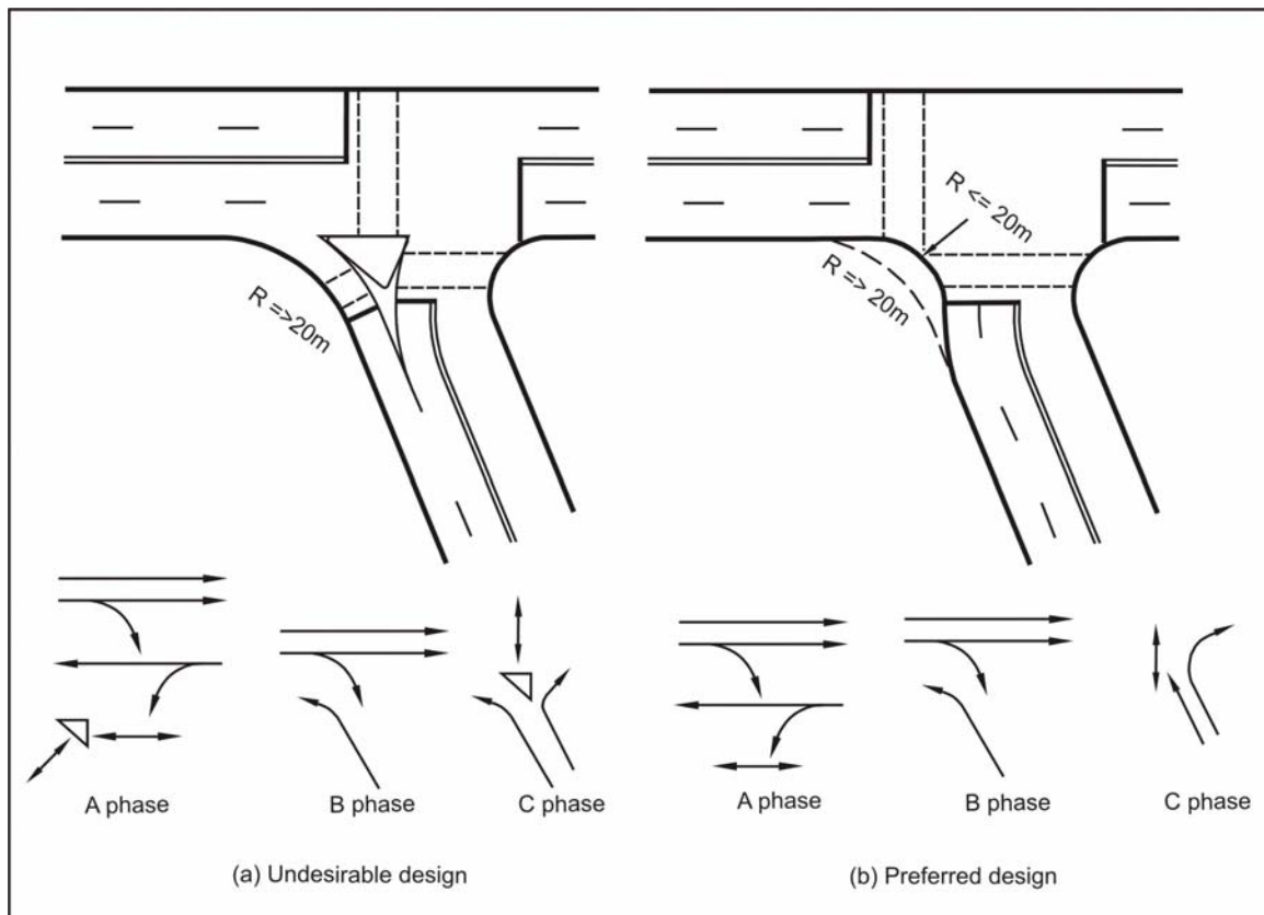
Figure 5.3 Eliminating corner island to improve design
