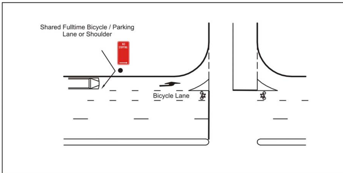
Figure 5.4 Typical pavement marking for bicycle lanes at intersections
