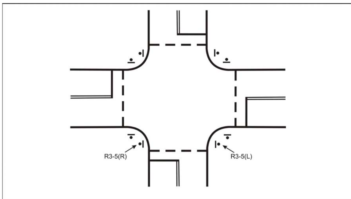
Figure 10.8 Position and Orientation of Scramble Crossing Sign
